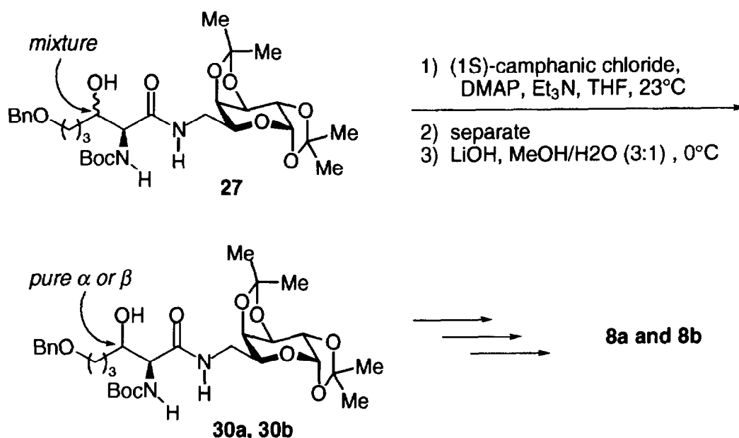
Scheme 5. Resolution of compound 8 .
