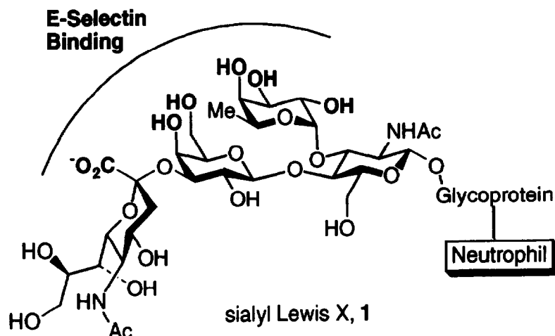
Figure 1. The structure of sialyl Lewis X showing the five functional groups essential for binding to E -selectin.
