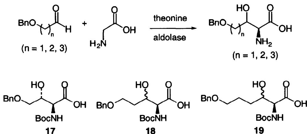
Scheme 2. Synthesis of amino acids 17–19.
