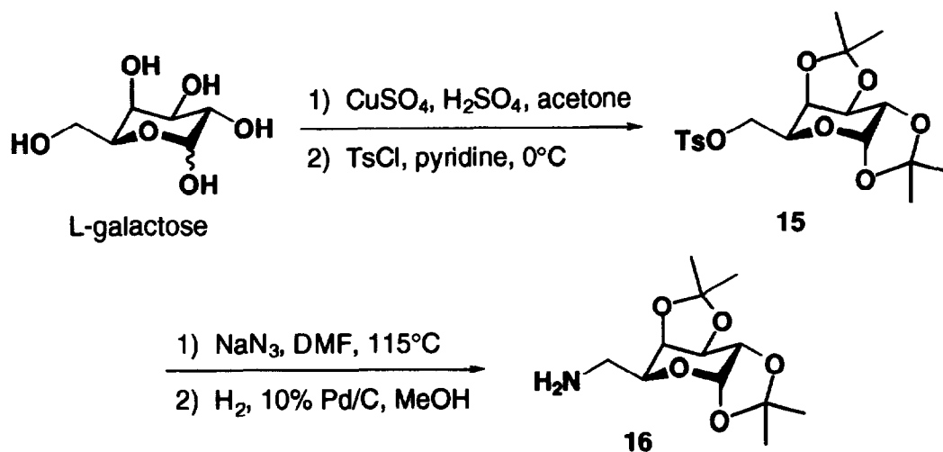
Scheme 1. Preparation of the galactose amine core.
