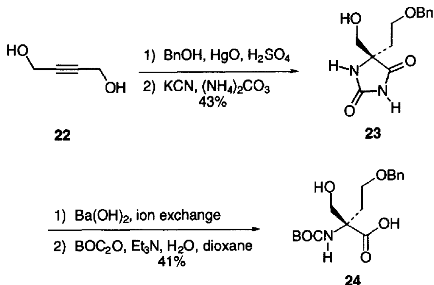
Scheme 4. Synthesis of amino acid 24.
