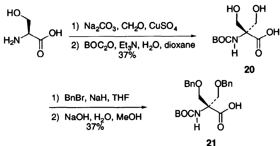
Scheme 3. Synthesis of dihydroxy amino acid 21.
